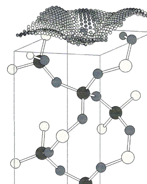
Figure 1. COSMO charges for a hydroxylated \alpha -Quartz (0001) surface. Silicon atoms are displayed as dark balls, oxygen atoms as light color balls.
